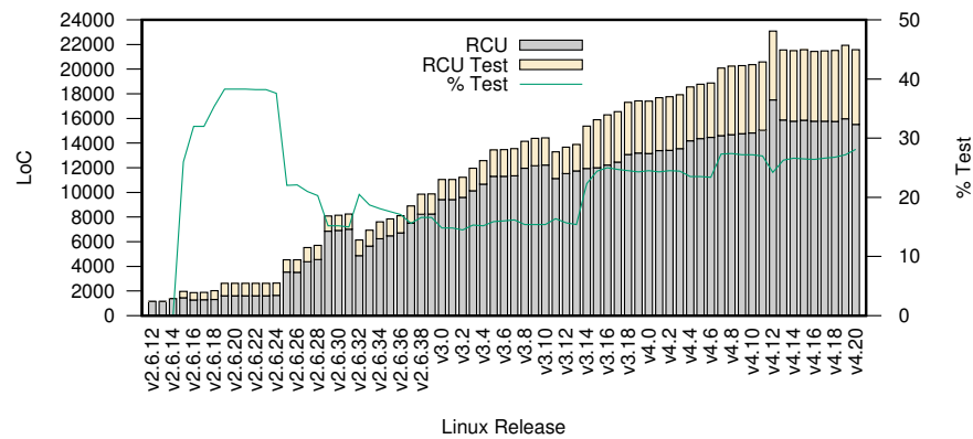
Figure 12.4: Linux-Kernel RCU Test Code
