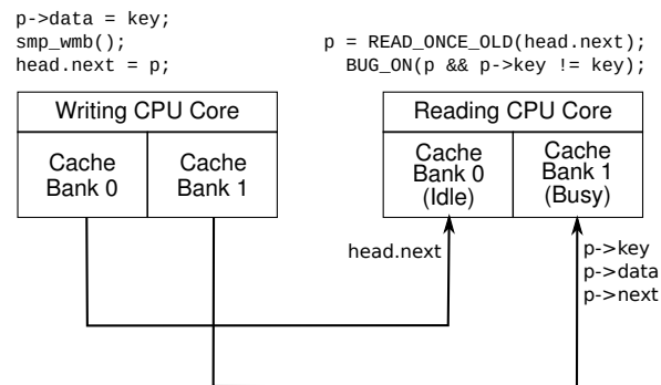
Figure 15.15: Why smp_read_barrier_depends() is Required in Pre-v4.15 Linux Kernels
