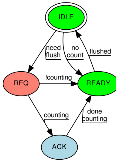
Figure 5.7: Signal-Theft State Machine
