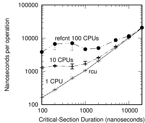
Figure 9.29: Response Time of RCU vs. Reference Counting
