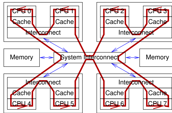
Figure 5.2: Data Flow For Global Atomic Increment
