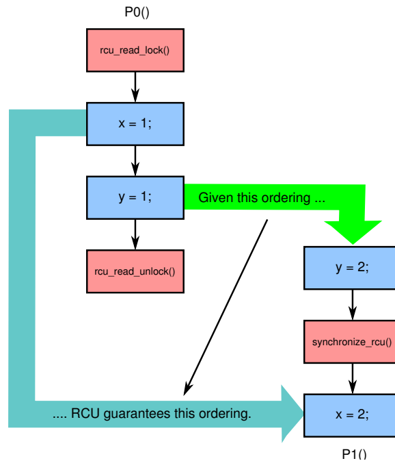
Figure 9.11: RCU Reader and Later Grace Period
