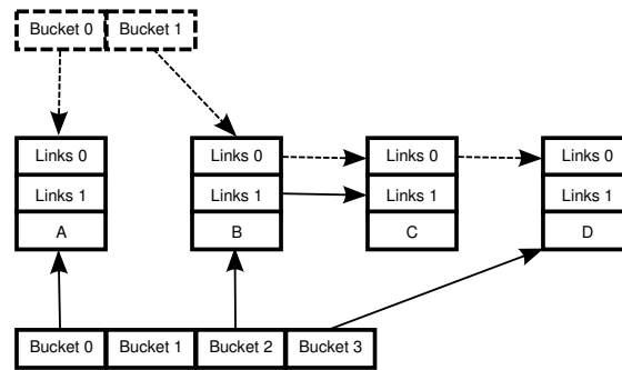
Figure 10.17: Growing a Double-List Hash Table, State (c)
