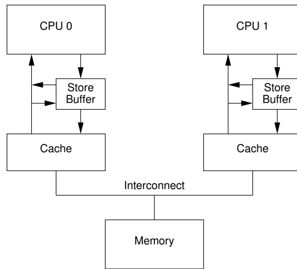
Figure C.6: Caches With Store Forwarding
