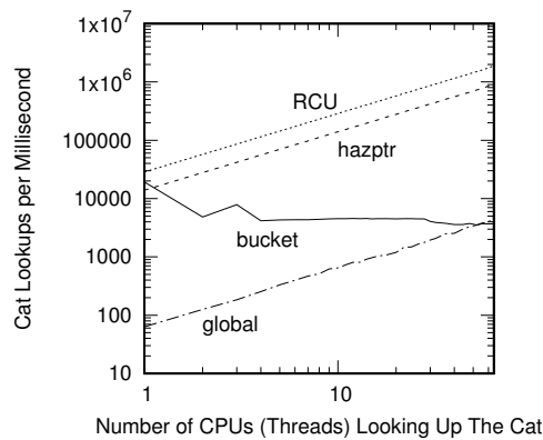
Figure 10.10: Read-Side Cat-Only RCU-Protected Hash-Table Performance For Schrödinger’s Zoo at 64 CPUs
