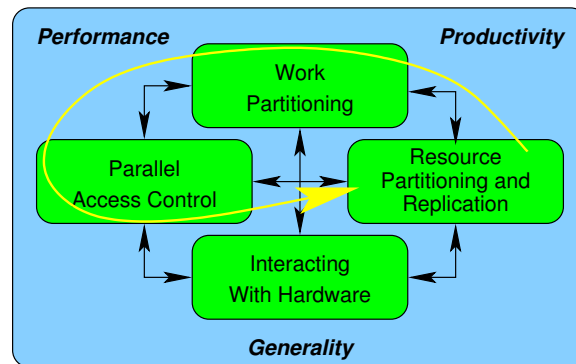
Figure 2.6: Ordering of Parallel-Programming Tasks
