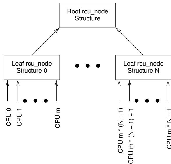
Figure 7.8: Locking Hierarchy
