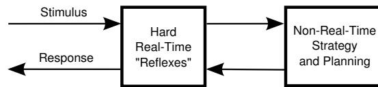
Figure 14.4: Real-Time Reflexes
