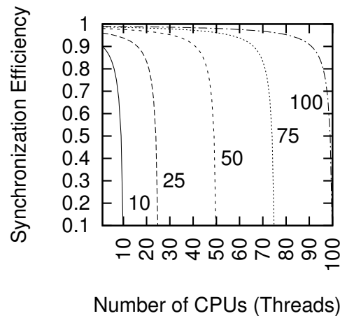
Figure 6.16: Synchronization Efficiency
