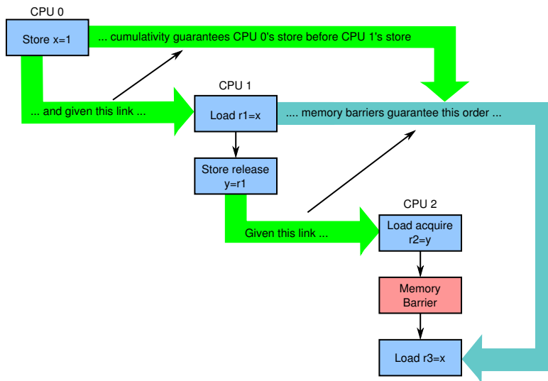
Figure 15.9: Cumulativeness
