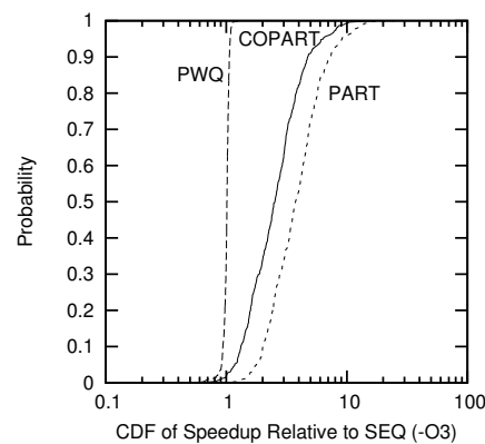
Figure 6.30: Partitioned Coroutines
