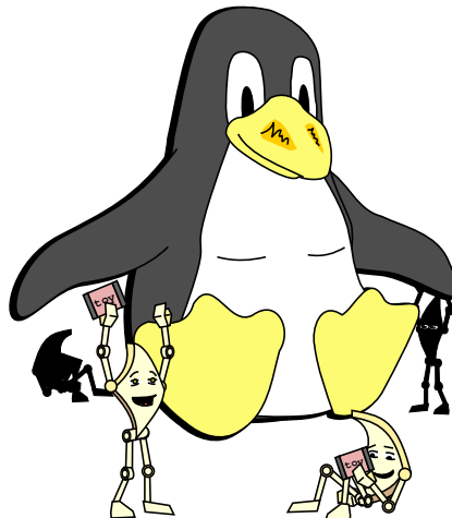
Figure 6.14: Data Locking
