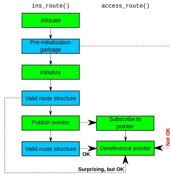
Figure 9.10: Publication/Subscription Constraints
