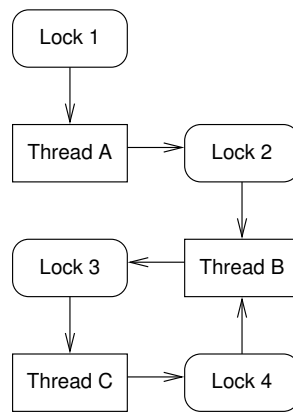
Figure 7.3: Deadlock Cycle
