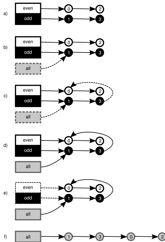
Figure 10.20: Shrinking a Relativistic Hash Table
