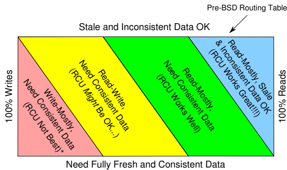
Figure 9.30: RCU Areas of Applicability
