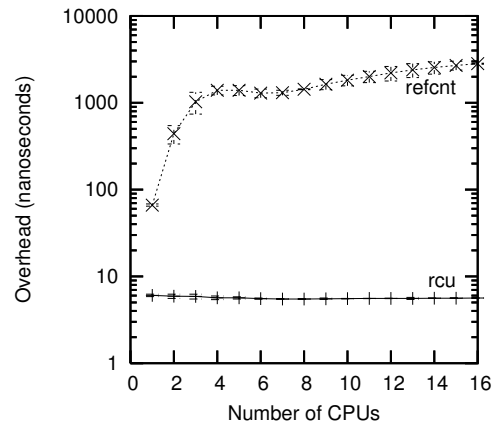
Figure 9.27: Performance of RCU vs. Reference Counting
