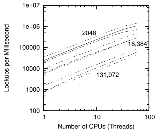
Figure 10.17: Overhead of Resizing Hash Tables Between 1024 and 2048 Buckets vs. Total Number of Elements
