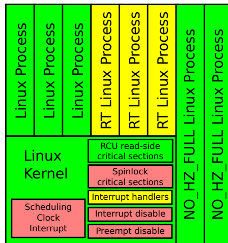
Figure 14.8: CPU Isolation
