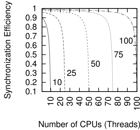
Figure 6.16: Synchronization Efficiency
