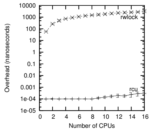
Figure 9.23: Performance Advantage of RCU Over Reader-Writer Locking
