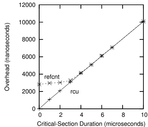
Figure 9.28: Response Time of RCU vs. Reference Counting
